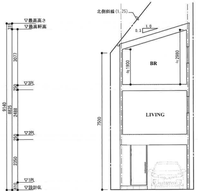
E-W SECTION
