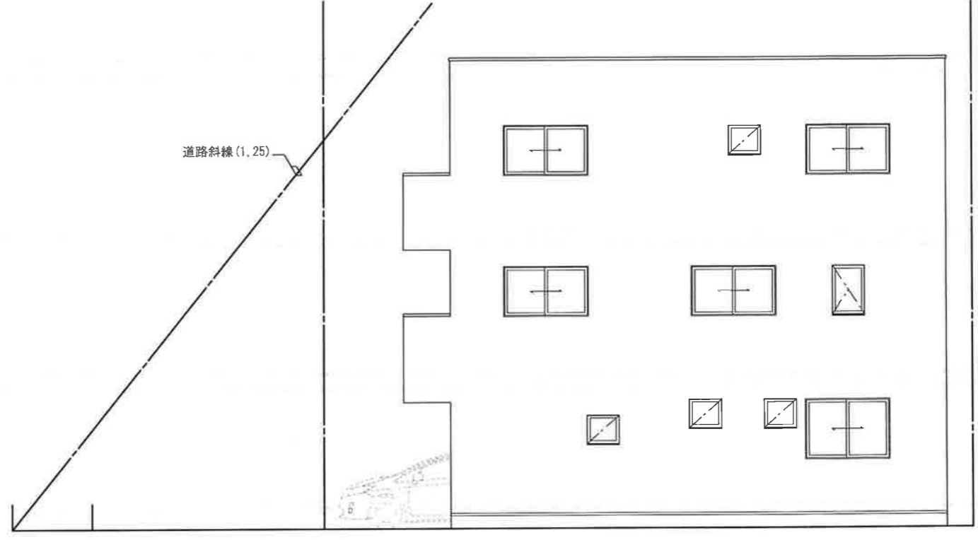
SOUTH ELEVATION
