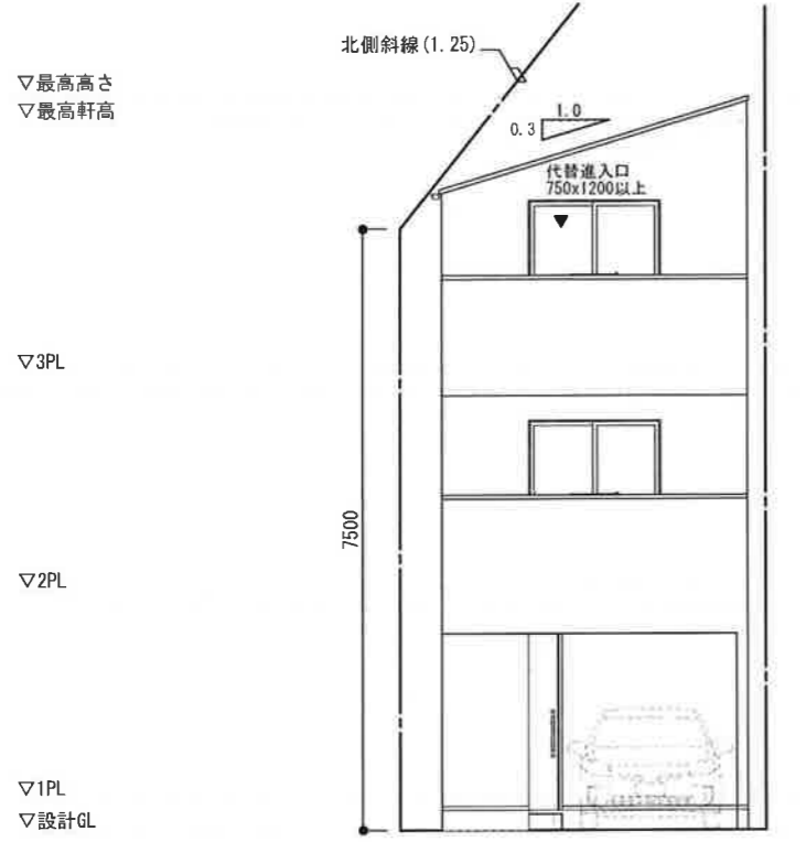
WEST ELEVATION
